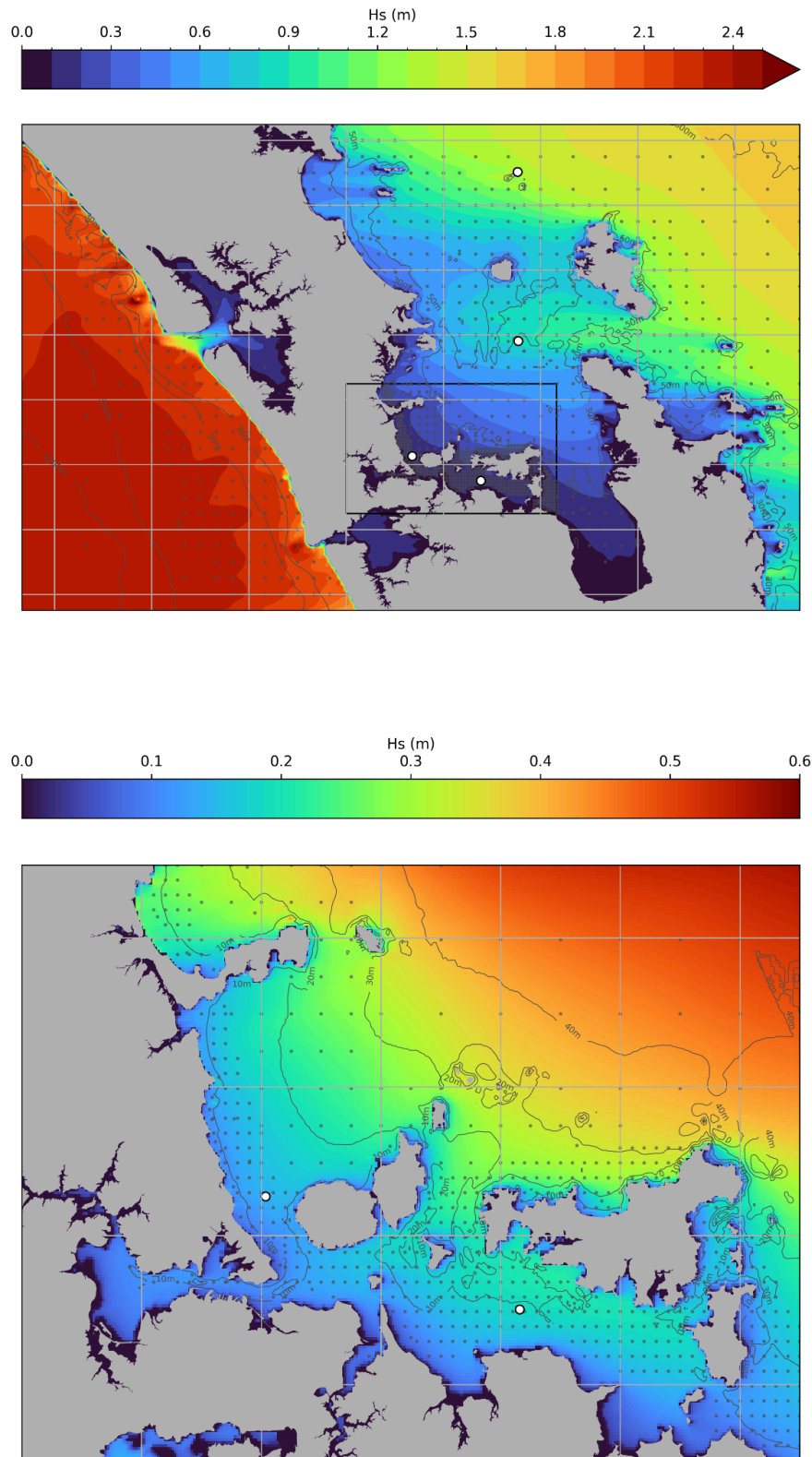
Figure 1. Significant wave height H_s from the (top) Auckland 1 km, and (bottom) Eastern Auckland 200 forecast domains averaged over a forecast cycle. Grey circles show the locations of spectra output. Rectangle indicates the location of the 200 m domain. White circles show the wave buoy locations used to validate the model.
