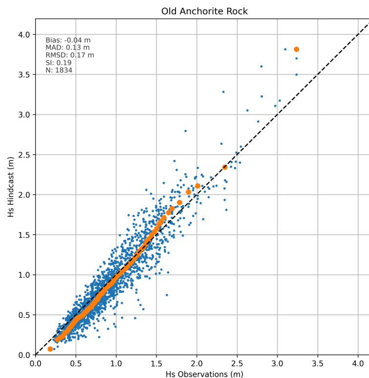
Figure 6. Scatter plot comparing hindcast and measured significant wave height H_s at Old Anchorite Rock. The orange markers represent the 0.01 quantiles, while the black dashed line denotes the equality line. Key statistics are shown in the upper left corner, including Bias, Mean Absolute Deviation (MAD), Root Mean Square Deviation (RMSD), Scatter Index (SI), and the number of data points (N).
