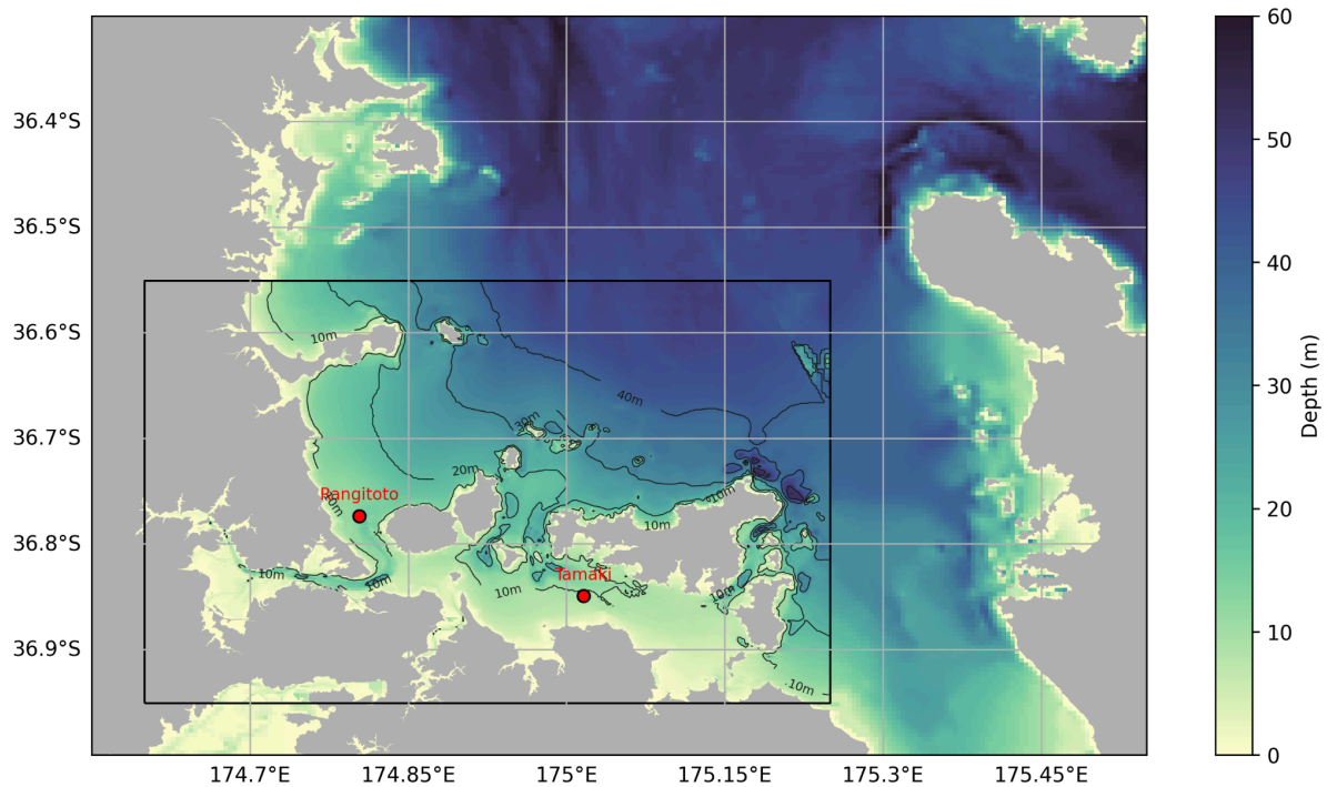
Figure 7. Bathymetry map of the Hauraki Gulf showing the locations of the two recent wave buoy observation sites. Black rectangle shows the extent of the 200 m grid.
