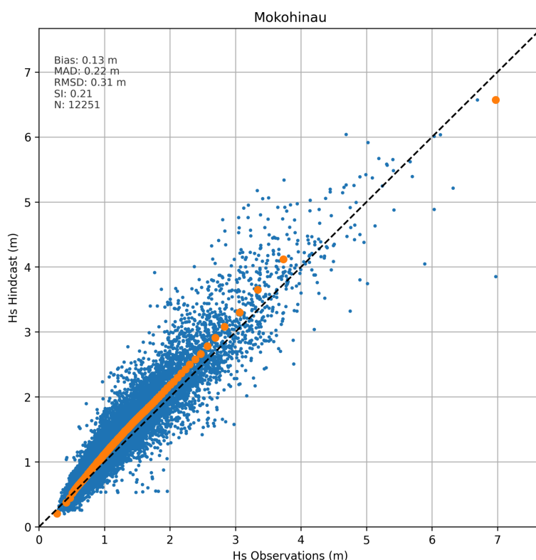
Figure 4. Scatter plot comparing hindcast and measured significant wave height H_s at Mokohinau. The orange markers represent the 0.01 quantiles, while the black dashed line denotes the equality line. Key statistics are shown in the upper left corner, including Bias, Mean Absolute Deviation (MAD), Root Mean Square Deviation (RMSD), Scatter Index (SI), and the number of data points (N).
