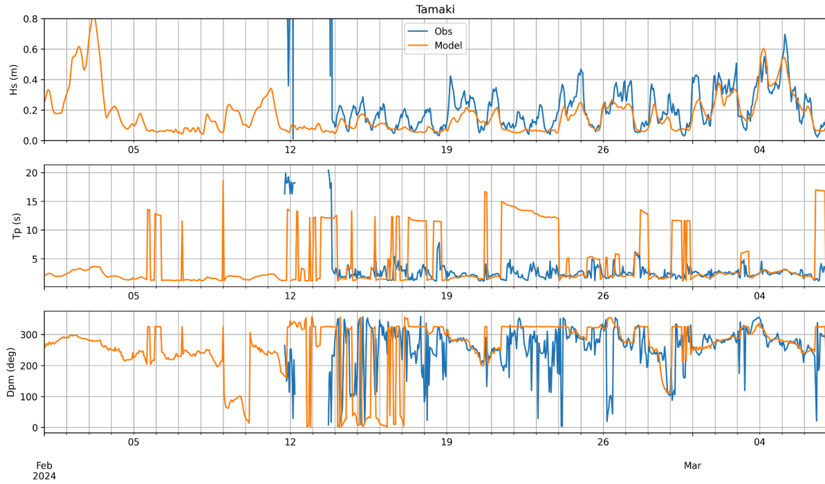
Figure 10. Time series comparison of observed (blue) and modelled (orange) wave parameters at Tamaki from February to March 2024. The plots show (top) significant wave height H_s , (middle) peak wave period T_p , and (bottom) mean wave direction D_{pm} .
