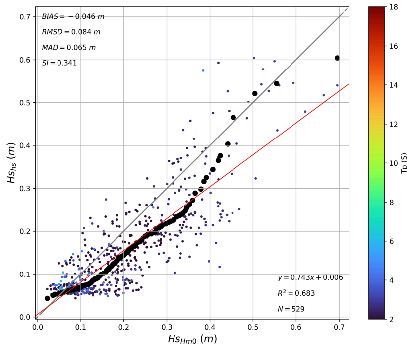
Figure 11. Scatter plot comparing hindcast and measured significant wave height H_s at Tamaki. Data points are coloured by peak wave period ( T_p ), with larger black circles representing the 0.01 quantiles, the red line the linear regression and the black line the equality. Key statistical metrics are displayed in the upper left corner, including Bias, Root Mean Square Deviation (RMSD), Mean Absolute Deviation (MAD), and Scatter Index (SI).
