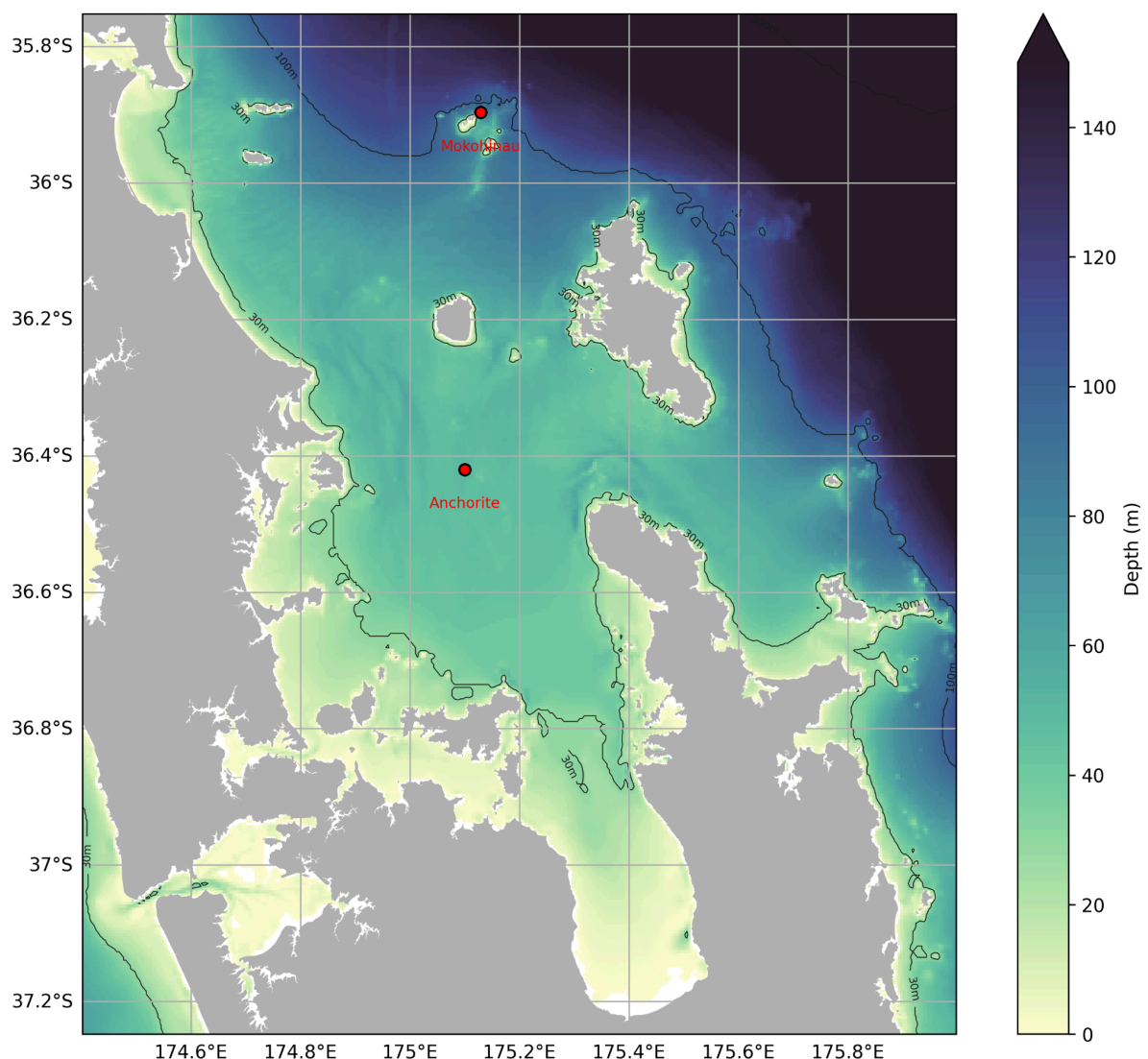
Figure 2. Bathymetry map of the Hauraki Gulf and adjacent coast showing the locations of the two historical wave buoy observation sites.
