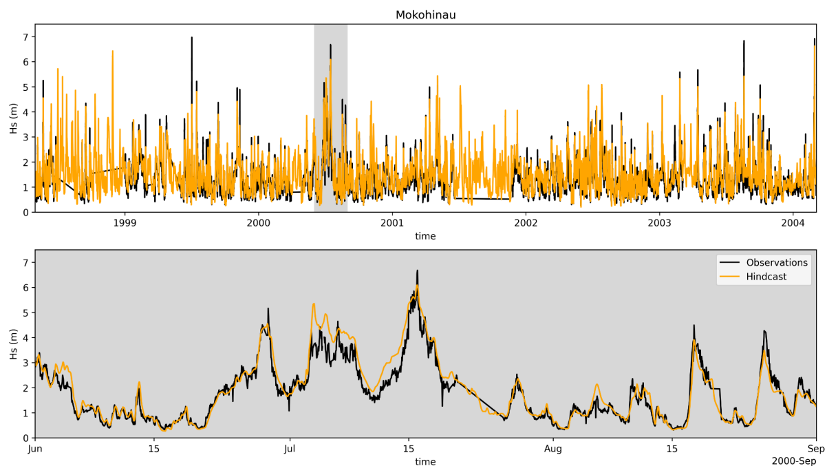
Figure 3. Time series of significant wave height H_s from the Mokohinau wave buoy and the wave hindcast, the shaded period is shown in detail at the bottom.
