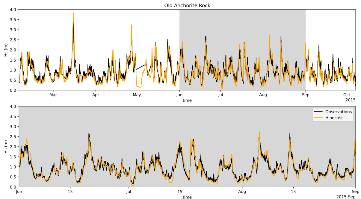
Figure 5. Time series of significant wave height H_s from the Old Anchorite Rock wave buoy and the wave hindcast, the shaded period is shown in detail at the bottom.
