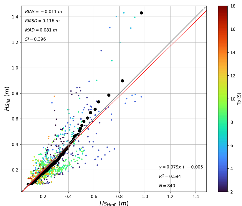
Figure 9. Scatter plot comparing hindcast and measured significant wave height H_s at Rangitoto. Data points are coloured by peak wave period ( T_p ), with larger black circles representing the 0.01 quantiles, the red line the linear regression and the black line the equality. Key statistical metrics are displayed in the upper left corner, including Bias, Root Mean Square Deviation (RMSD), Mean Absolute Deviation (MAD), and Scatter Index (SI).
