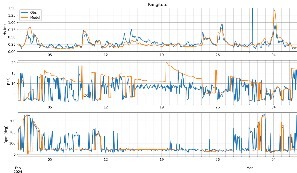
Figure 8. Time series comparison of observed (blue) and modelled (orange) wave parameters at Rangitoto from February to March 2024. The plots show (top) significant wave height H_s , (middle) peak wave period T_p , and (bottom) mean wave direction D_{pm} .
