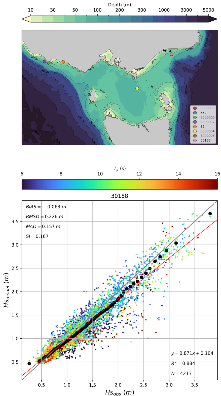
Figure 11. Hindcast validation at wave buoy ID 30188: (top) model depth map showing the location of historical buoys with the drifting buoy locations highlighted by the black dots, and (bottom) comparison between modelled and measured significant wave height H_s with colours representing the measured peak wave period, black circles the H_s quantiles and the red line the linear regression.
