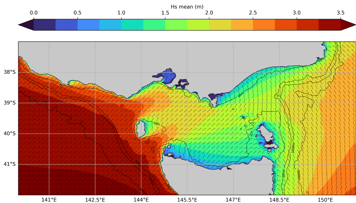
Figure 3. Mean significant wave height H_s from the 5 km Bass Strait domain for 1993-2023.
