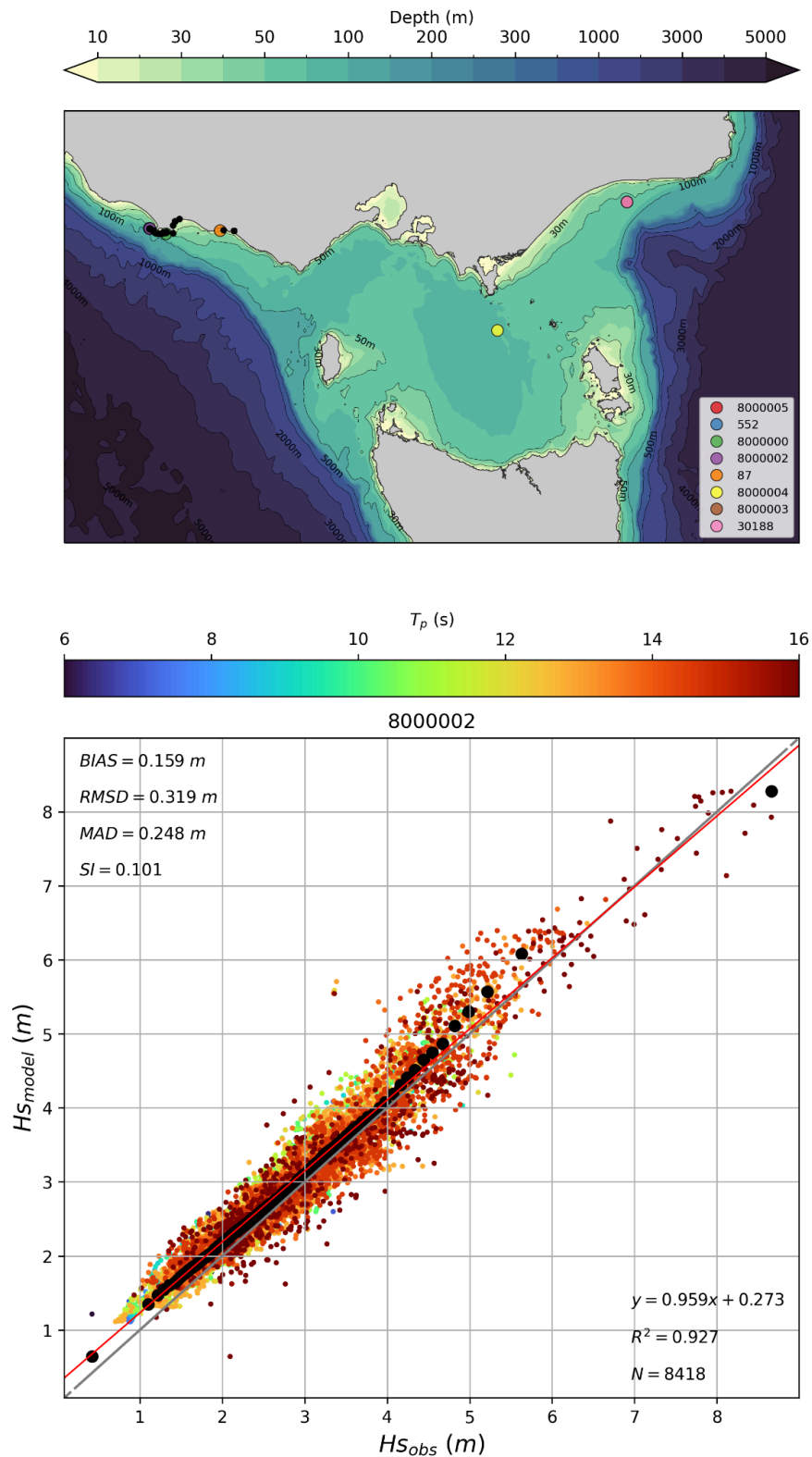
Figure 7. Hindcast validation at wave buoy ID 8000002: (top) model depth map showing the location of historical buoys with the drifting buoy locations highlighted by the black dots, and (bottom) comparison between modelled and measured significant wave height H_s with colours representing the measured peak wave period, black circles the H_s quantiles and the red line the linear regression.
