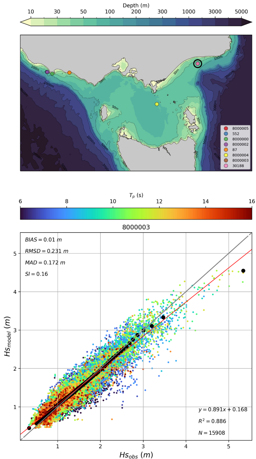
Figure 10. Hindcast validation at wave buoy ID 8000003: (top) model depth map showing the location of historical buoys with the current location highlighted by the black circle, and (bottom) comparison between modelled and measured significant wave height H_s with colours representing the measured peak wave period, black circles the H_s quantiles and the red line the linear regression.
