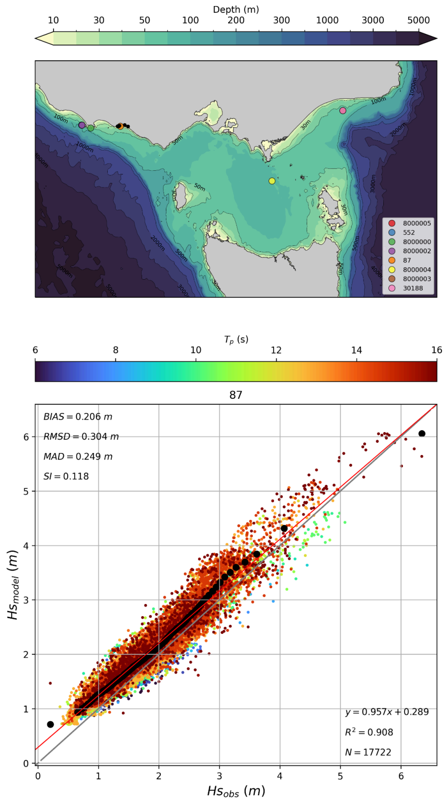
Figure 8. Hindcast validation at wave buoy ID 87: (top) model depth map showing the location of historical buoys with the drifting buoy locations highlighted by the black dots, and (bottom) comparison between modelled and measured significant wave height H_s with colours representing the measured peak wave period, black circles the H_s quantiles and the red line the linear regression.
