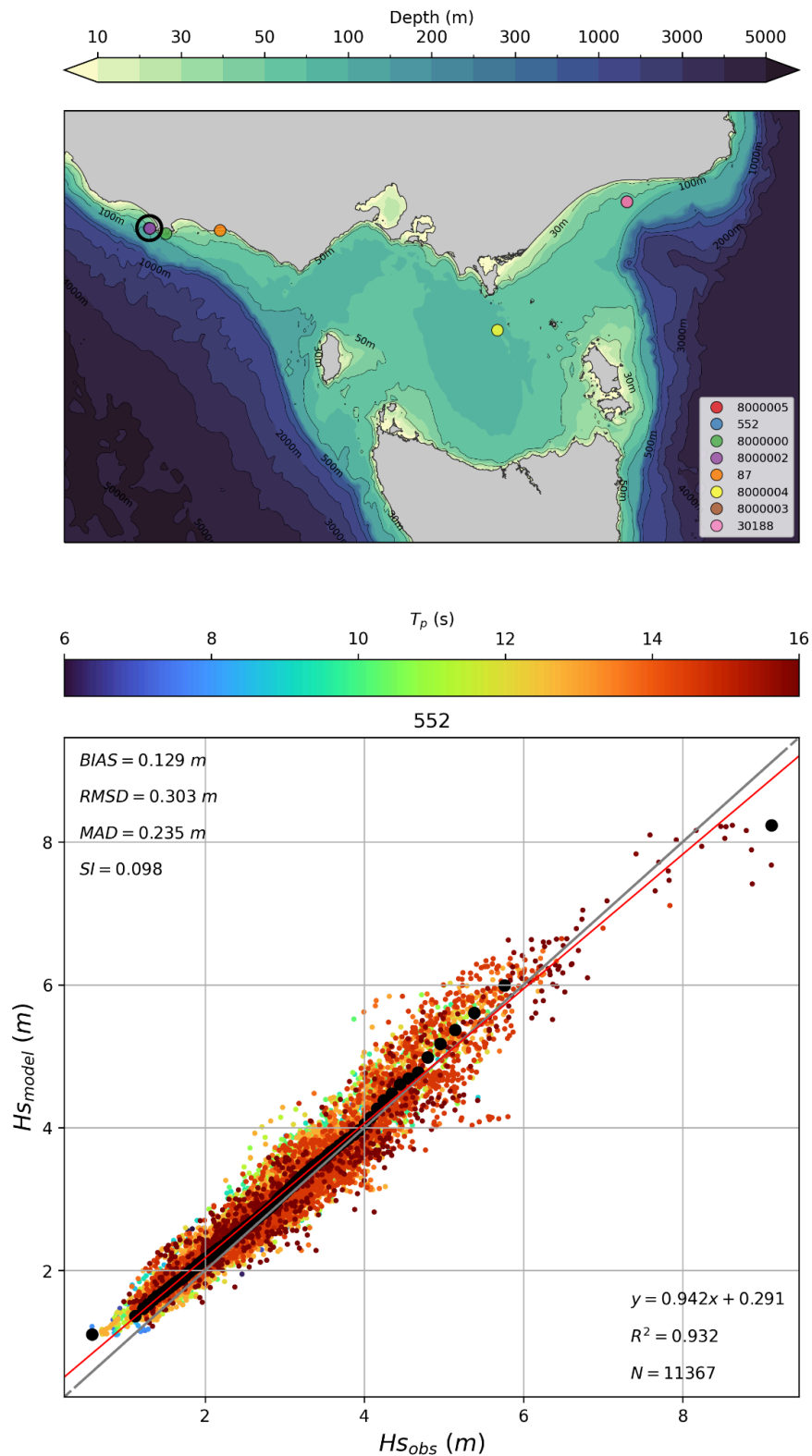
Figure 5. Hindcast validation at wave buoy ID 552: (top) model depth map showing the location of historical buoys with the current location highlighted by the black circle, and (bottom) comparison between modelled and measured significant wave height H_s with colours representing the measured peak wave period, black circles the H_s quantiles and the red line the linear regression.
