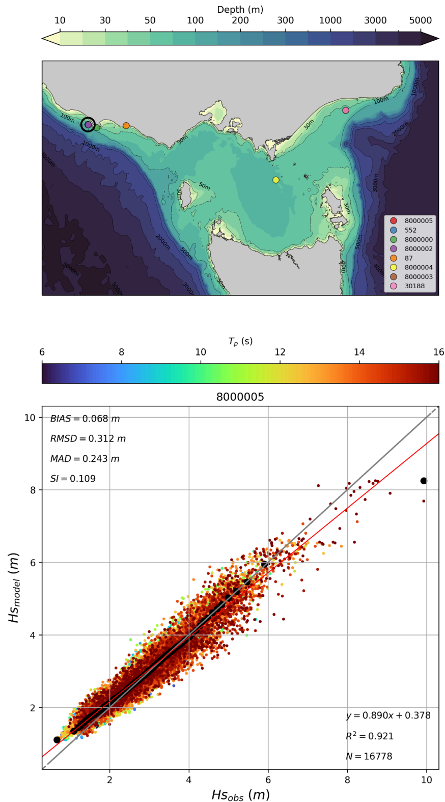
Figure 4. Hindcast validation at wave buoy ID 8000005: (top) model depth map showing the location of historical buoys with the current location highlighted by the black circle, and (bottom) comparison between modelled and measured significant wave height H_s with colours representing the measured peak wave period, black circles the H_s quantiles and the red line the linear regression.
