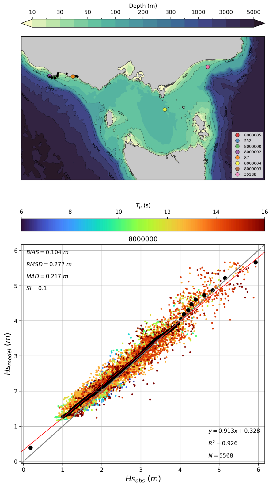
Figure 6. Hindcast validation at wave buoy ID 8000000: (top) model depth map showing the location of historical buoys with the drifting buoy locations highlighted by the black dots, and (bottom) comparison between modelled and measured significant wave height H_s with colours representing the measured peak wave period, black circles the H_s quantiles and the red line the linear regression.
