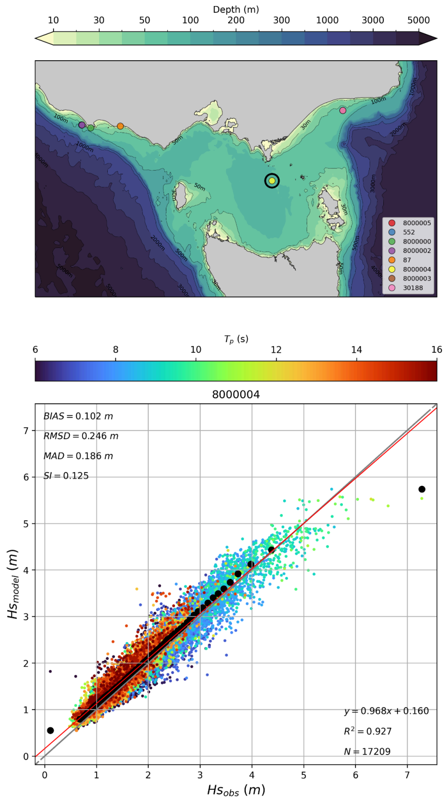
Figure 9. Hindcast validation at wave buoy ID 8000004: (top) model depth map showing the location of historical buoys with the current location highlighted by the black circle, and (bottom) comparison between modelled and measured significant wave height H_s with colours representing the measured peak wave period, black circles the H_s quantiles and the red line the linear regression.
