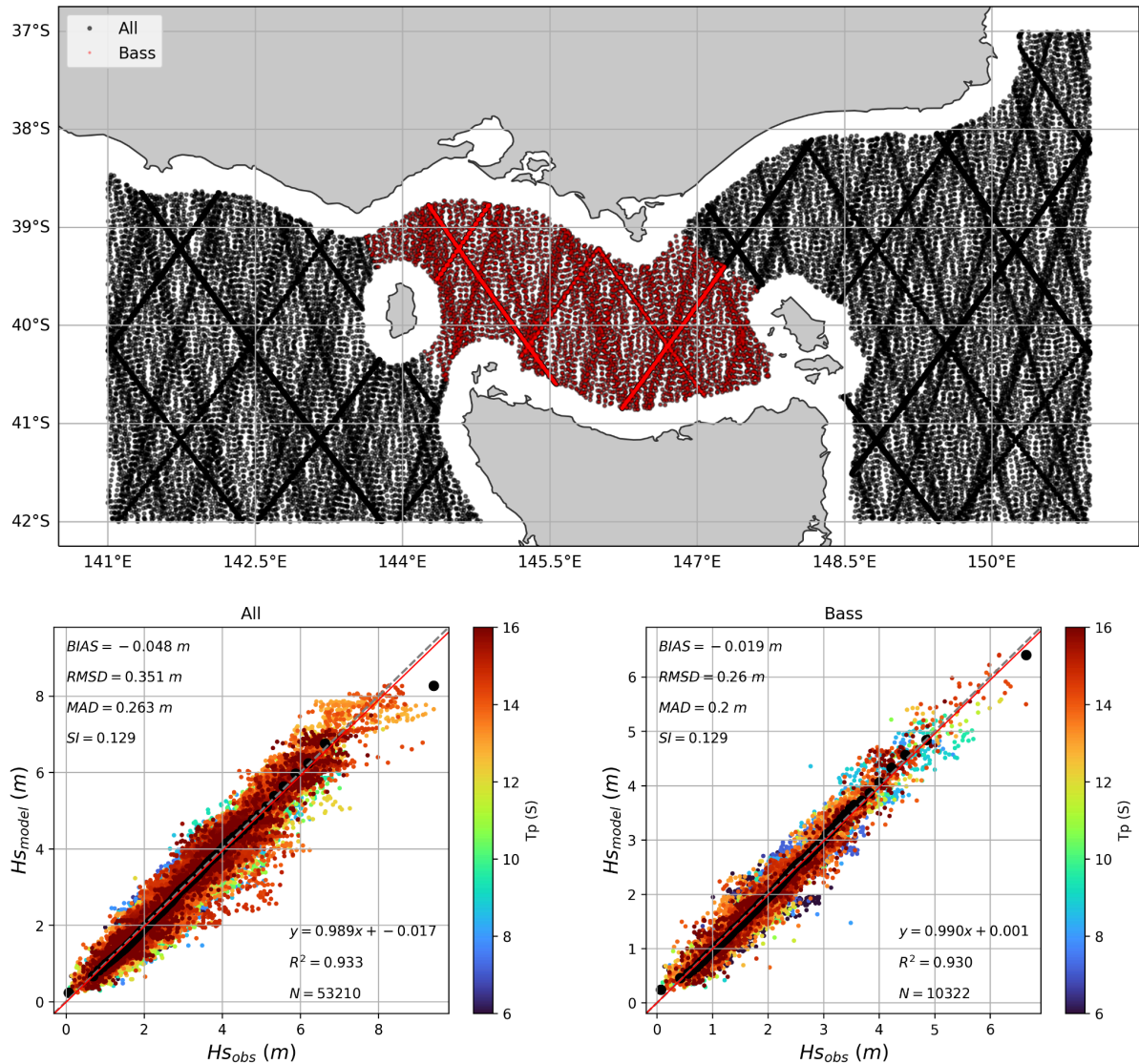
Figure 2. Validation of model significant wave height H_s against satellite altimeters for 2016. Results are presented for the approximate area of the 5 km domain and for the sheltered region inside the Bass Strait (black and red dots on the map, respectively).
