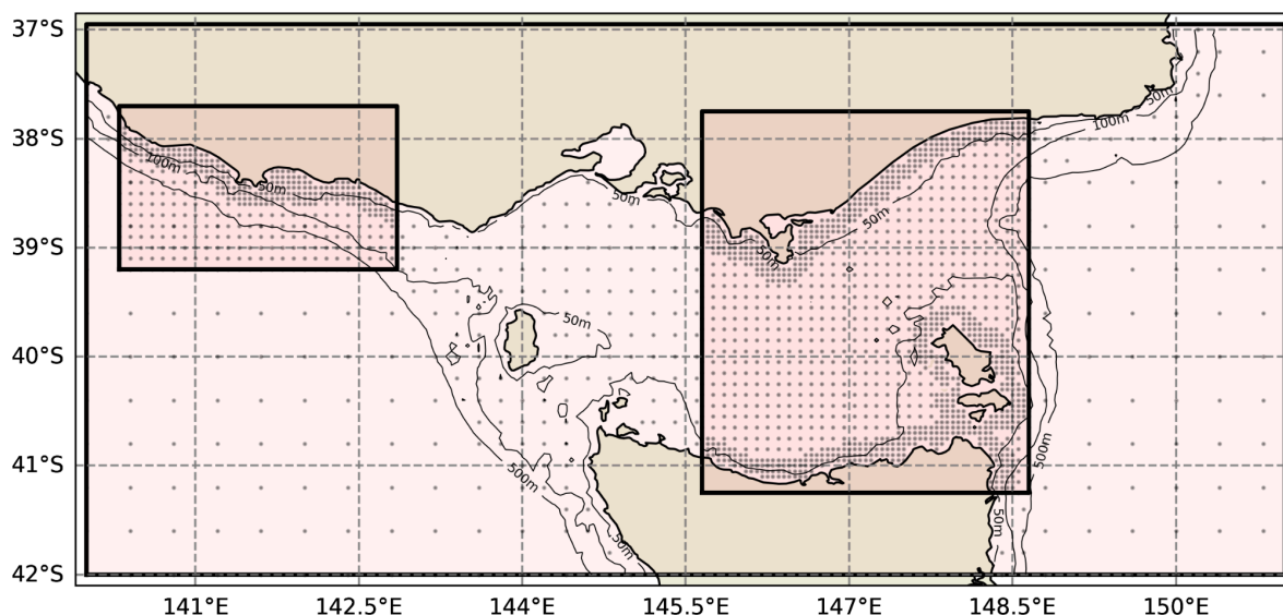
Figure 1. Wave model domains with spectra output locations represented by the dots.
